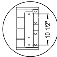
VIEW A-A FOOT PAD
