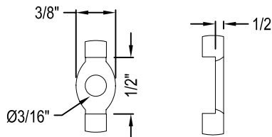
COINING DETAIL
